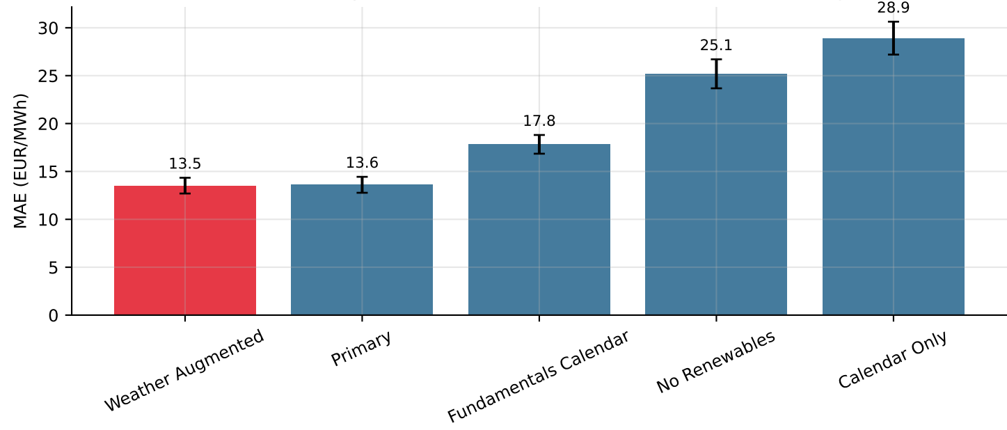
Feature-family ablations under an identical walk-forward design
